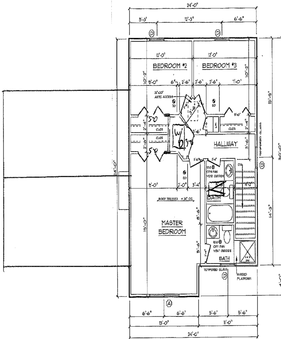
SECOND FLOOR PLAN ~ 1/4" = 1'-0"
