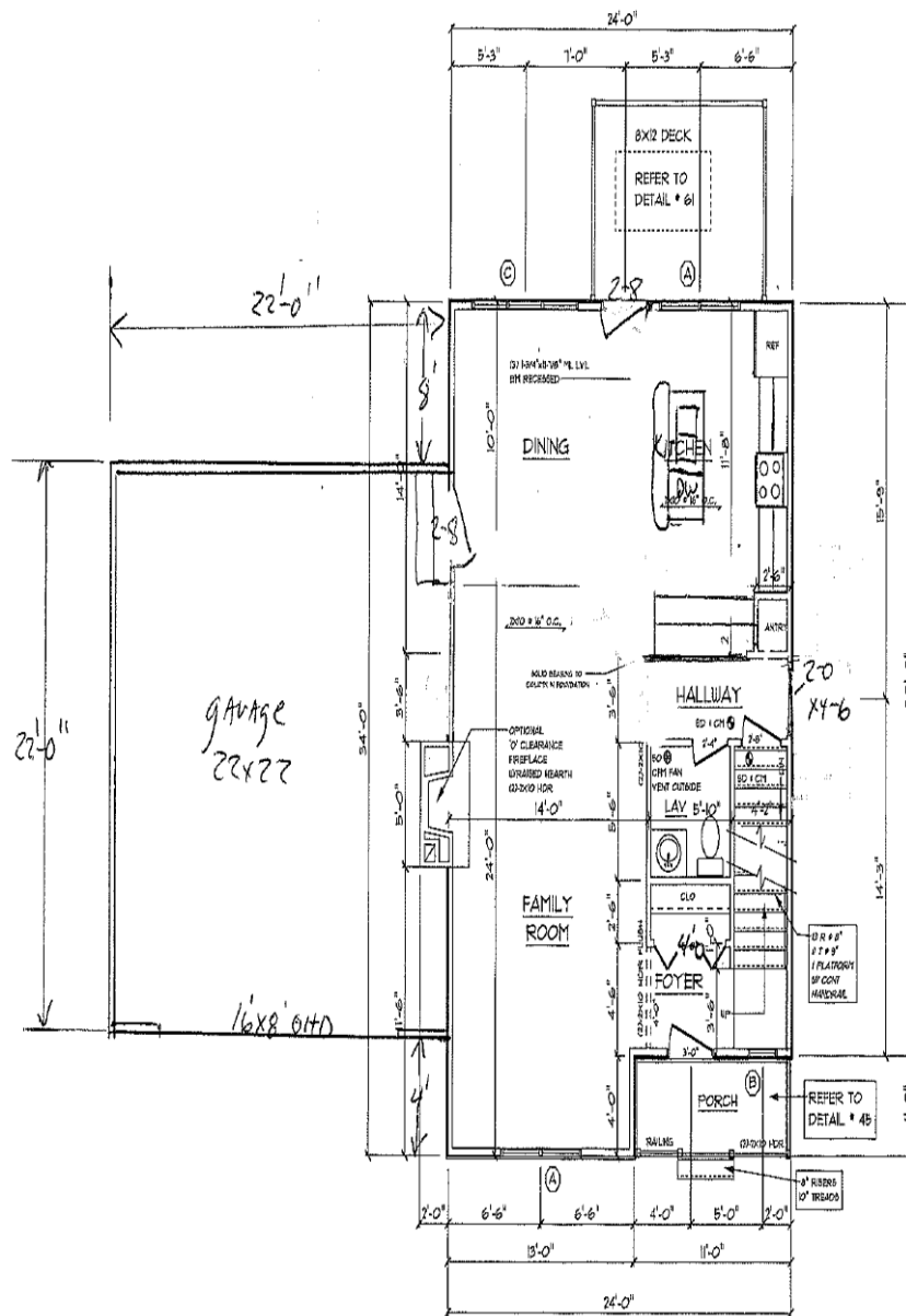
FIRST FLOOR PLAN ~ 1/4" = 1'-0"
